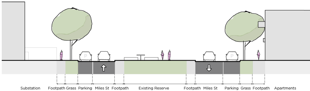
Existing Section, looking East
