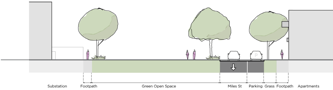
Proposed Section, looking East
